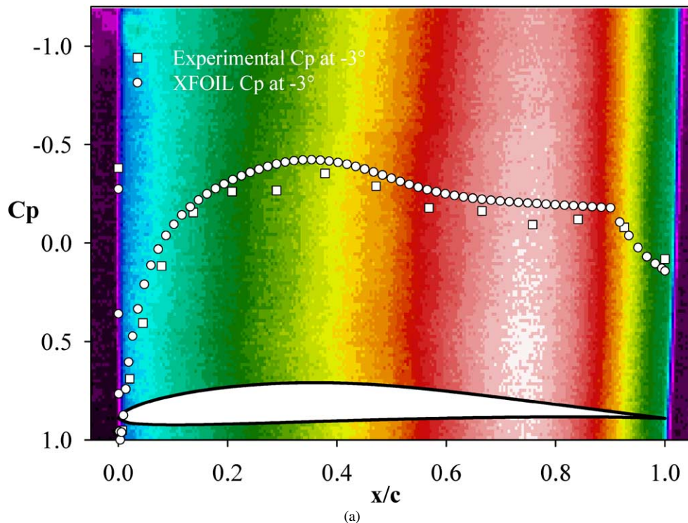
Fig. 15. Experimental and numerical C_p superimposed on the thermographic results.
